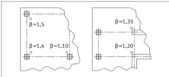
1) corner support, 2) edge support, 3) internal support, 4) wall end, 5) wall corner
